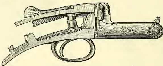
Mechanism of Hammerless Rook Rifle.
